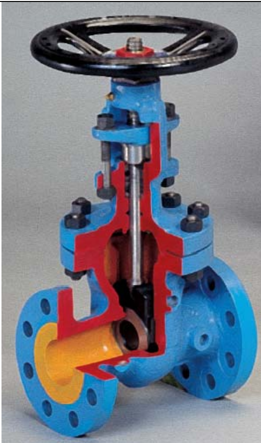
Gate Valve
